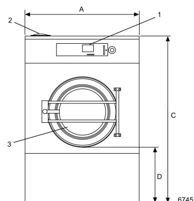
Front W4280X, W4350X
